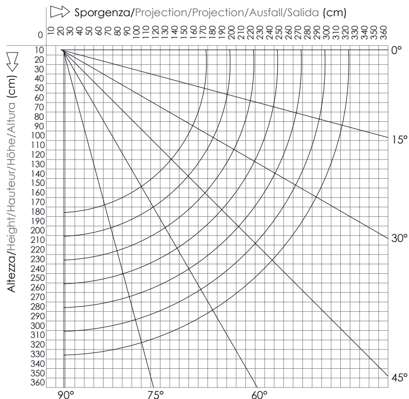
Montaggio a parete con staffa estrusa Wall installation with extruded bracket
